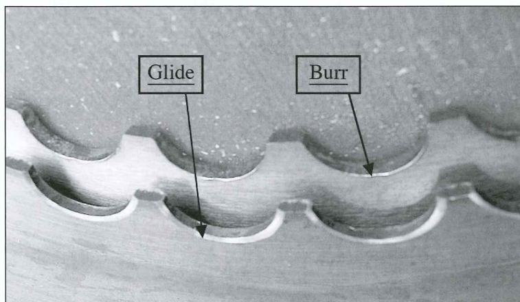
This illustration shows two #3 retec saws, one with the burr from contact with the arbor, the second with the Glide installed.
